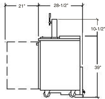
BM23C End
