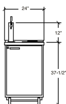
BM23C Front
