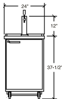
BM23 Front
