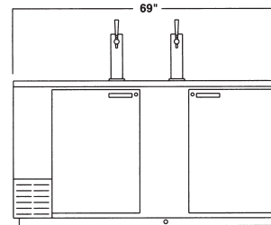
DD68 Front
