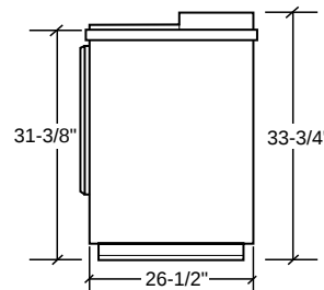
DW49, 64, 79, 94 Common End View
