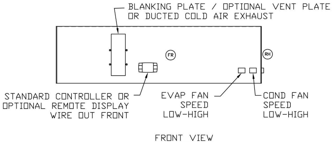
1800H CONTROL AND OPTIONAL FEATURE LOCATIONS UNIT FRONT AND TOP
