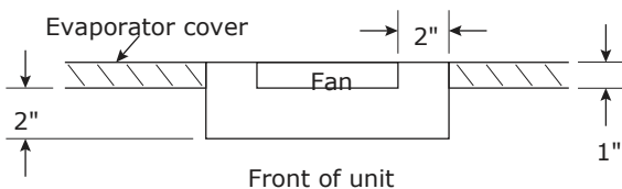
Internal Air Flow And Unit Ventilation Diagram Fan (top view)
