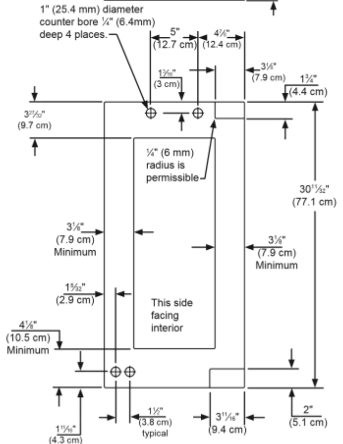
Figure 17 Left Hand Hinged Door 15" (38.1 cm) Wide Appliance
