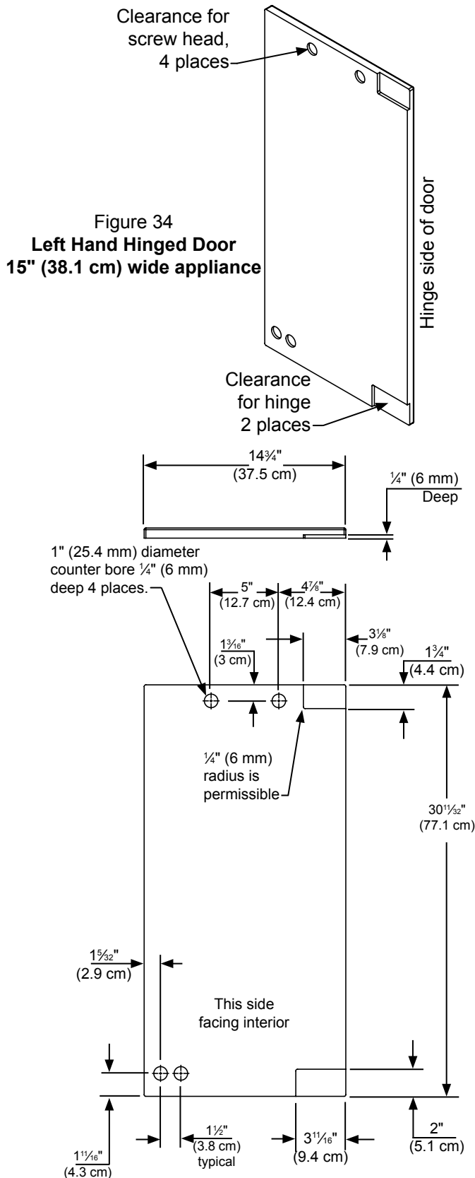
Figure 35 Left Hand Hinged Door 15" (38.1 cm) Wide Appliance
